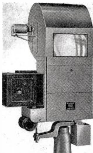
SCOPHONY Ltd., London firm, has developed this television projector for public halls. It projects an image 6 x 5 feet in black and white and resembles an ordinary film projector.
